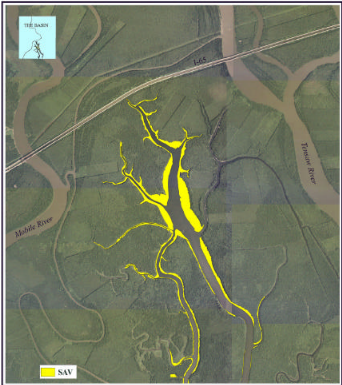
Figure 4-8. SAV in McReynolds Lake during 2002.
