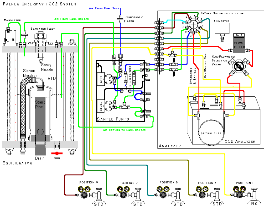
Figure 2: Diagram of the underway p\text{CO}_2 system used for surface water p\text{CO}_2 measurements during NBP04-03 which is essentially identical to the Gould System.
