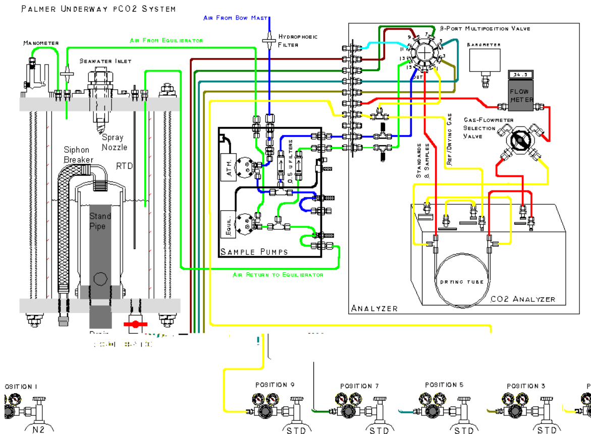
Figure 2: Diagram of the underway p\text{CO}_2 system used for surface water p\text{CO}_2 measurements during NBP04-03 which is essentially identical to the Gould System.
