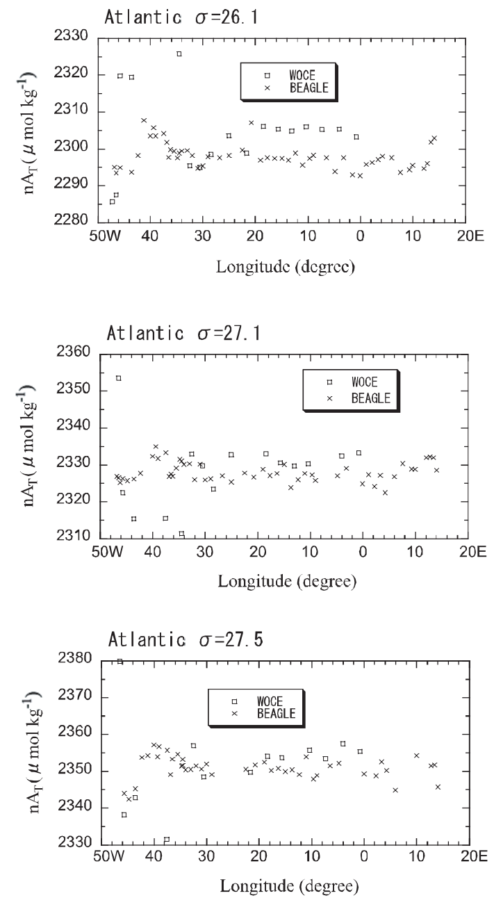
Figure 3.6.6. Comparisons of A_T measured in the BEAGLE with A_T calculated from C_T and p\text{CO}_2 measured along the WOCE A10 on isopycnal surfaces of 26.1 \sigma_\theta (top panel), 27.1 \sigma_\theta (middle panel) and 27.5 \sigma_\theta (bottom panel).
