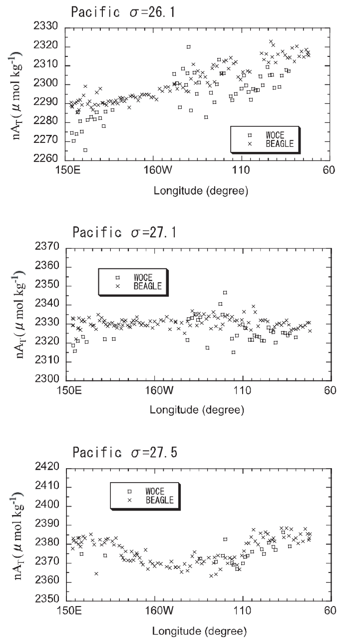
Figure 3.6.5. Comparisons of A_T measured in the BEAGLE with A_T calculated from C_T and p\text{CO}_2 measured along the WOCE P6 on isopycnal surfaces of 26.1 \sigma_\theta (top panel), 27.1 \sigma_\theta (middle panel) and 27.5 \sigma_\theta (bottom panel).
