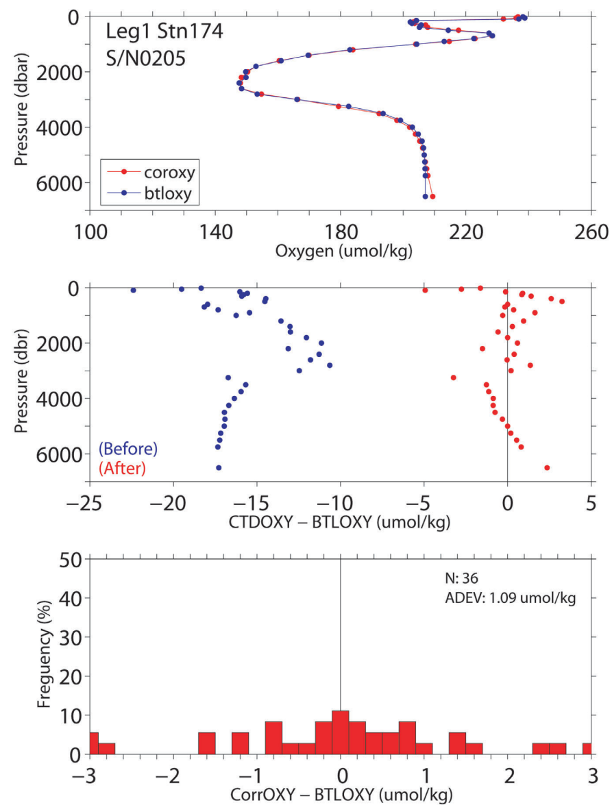
Figure 3.1.20. An example of difference between the CTD oxygen and the bottle oxygen (leg 1, P06_174) for secondary oxygen sensor (S/N 0205). Upper panel shows vertical profile of bottle oxygen (blue) and calibrated CTD oxygen (red). Middle panel shows vertical distribution of the difference (blue: before the calibration, red: after the calibration). Lower panel shows histogram of the difference after the calibration.
