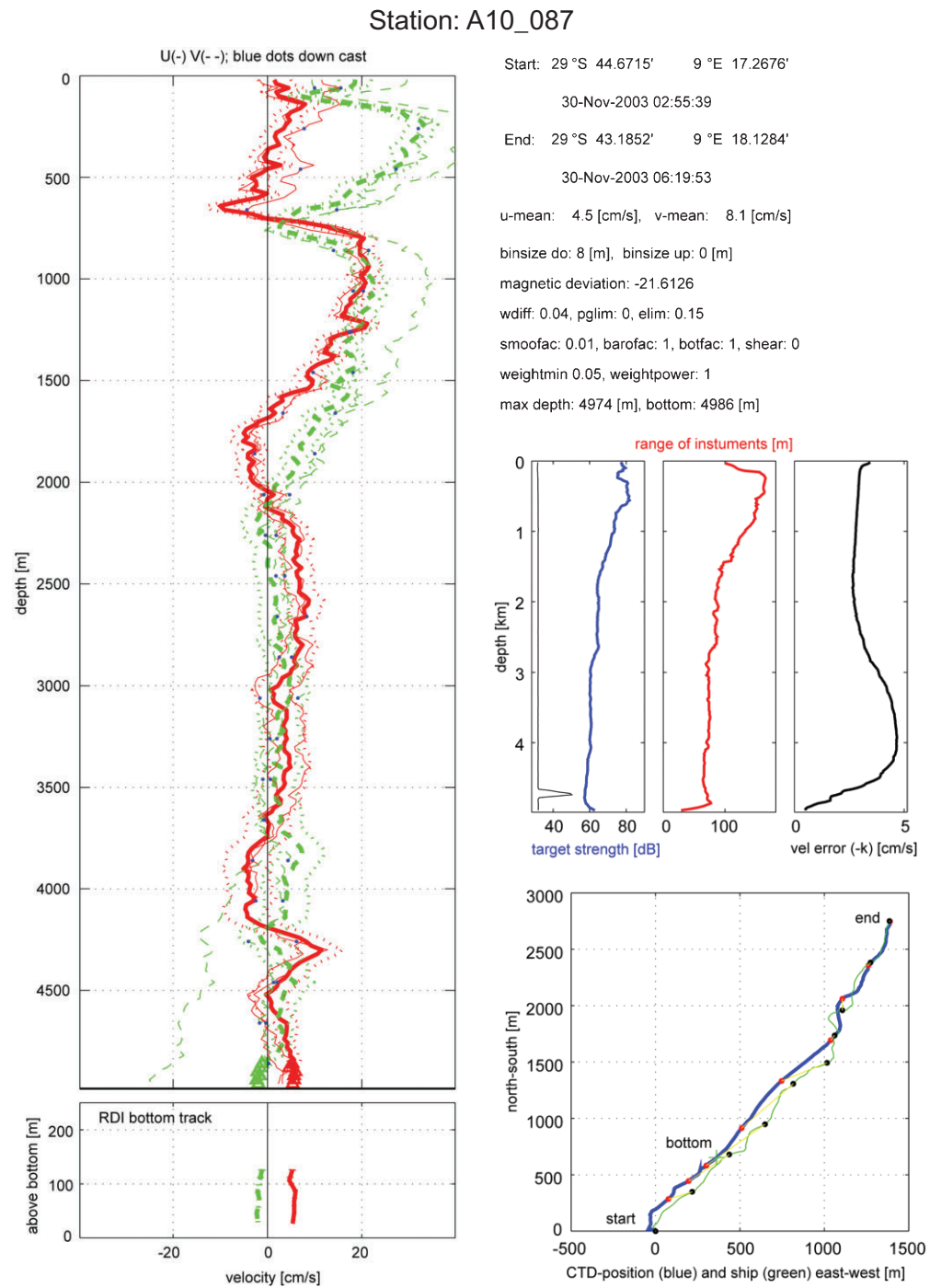
Figure 3.8.1. Vertical profiles of velocity at station A10_87.
