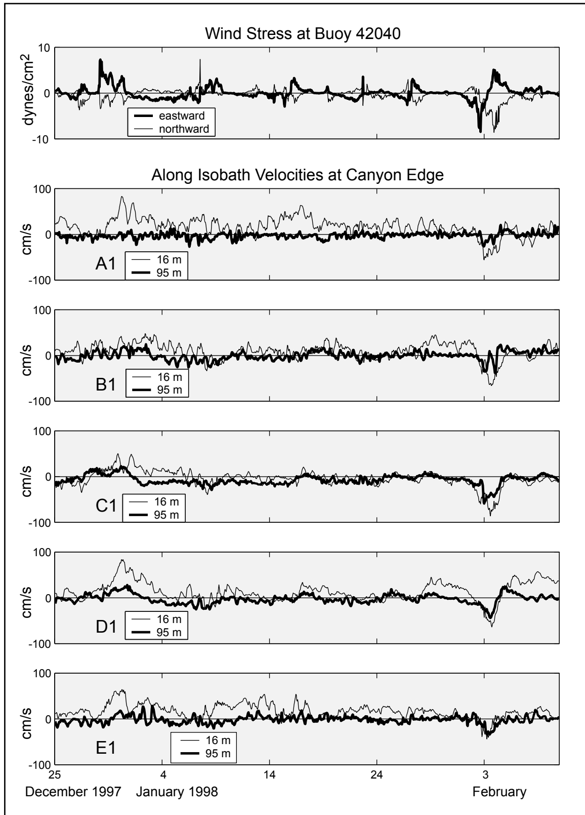
Figure 6.4-16. Near-bottom and near-surface, along-isobath velocities measured at the canyon edge moorings during the winter of 1997-1998.
