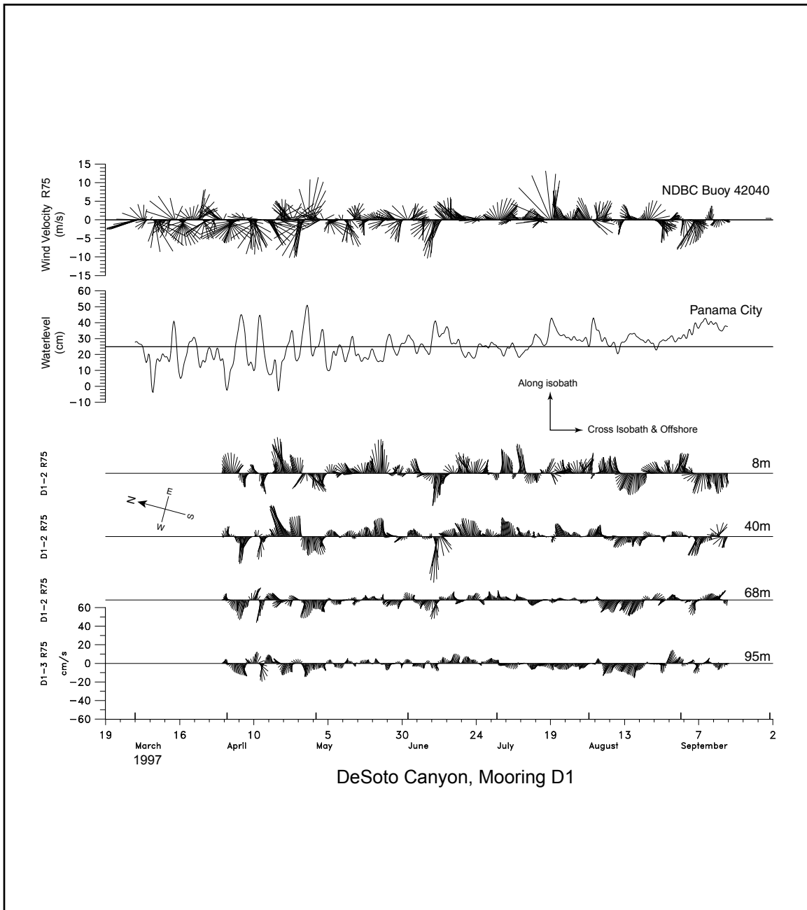
Figure 6.2-1a. Subtidal current vectors between 8 to 95m at mooring site D1 during March to September 1997 together with subtidal winds from buoy 42040, located near the A mooring line, and coastal sea level at Panama City, FL. See notations for directions of velocity vectors relative to isobaths and geographic frame-of-reference.
