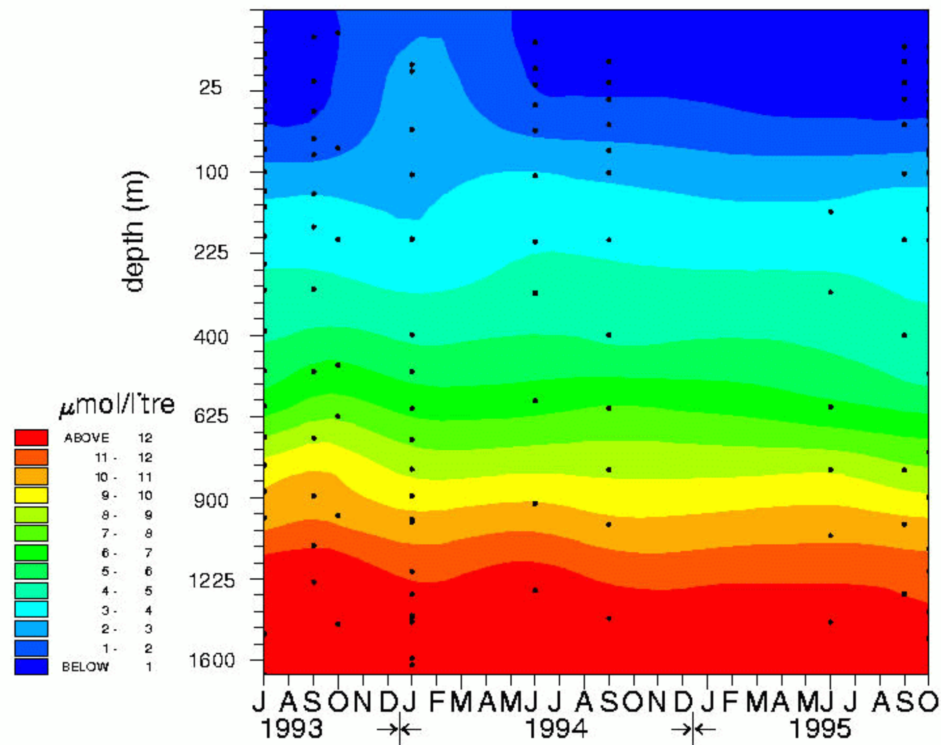
Time Series for Silicate at OMEX2 Station
